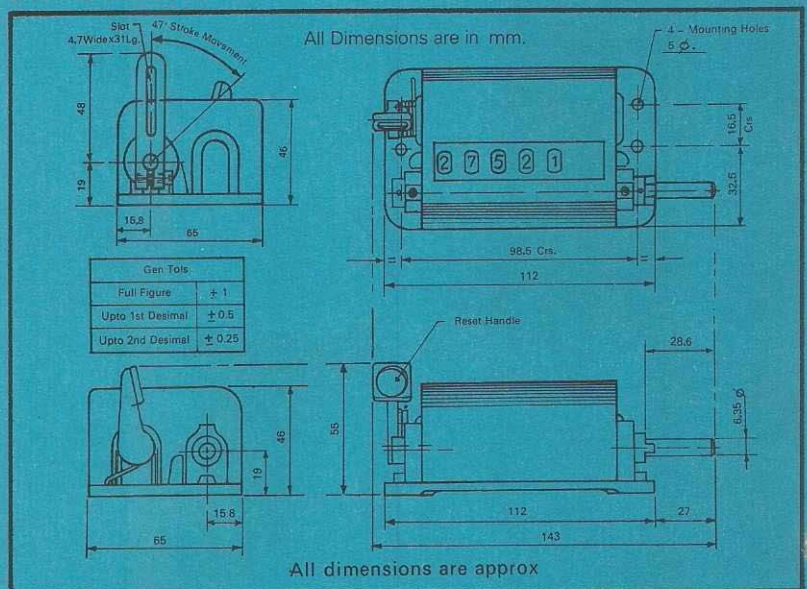
Loom Counter (Senior)-SL
